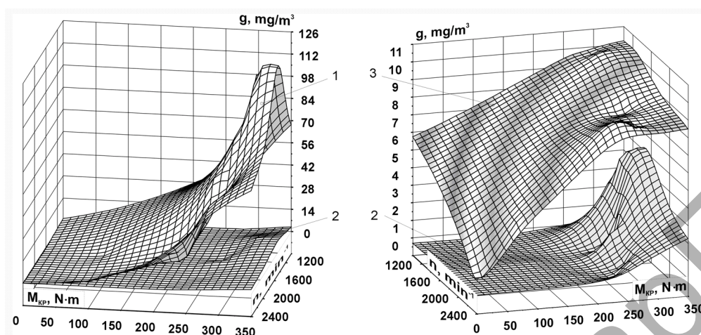
1 — the standard gas-outlet system; 2 — gas outlet system with PCR; 3 — the requirements of EURO-3 standard recalculated in operation conditions of diesel Д-243; g — the concentration of heavy particles in diesel EG, \text{mg}/\text{m}^3 ; n — the frequency of crankshaft rotation, \text{min}^{-1} ; M_{\text{кр}} — the twisting moment of engine, \text{H} \cdot \text{m}
