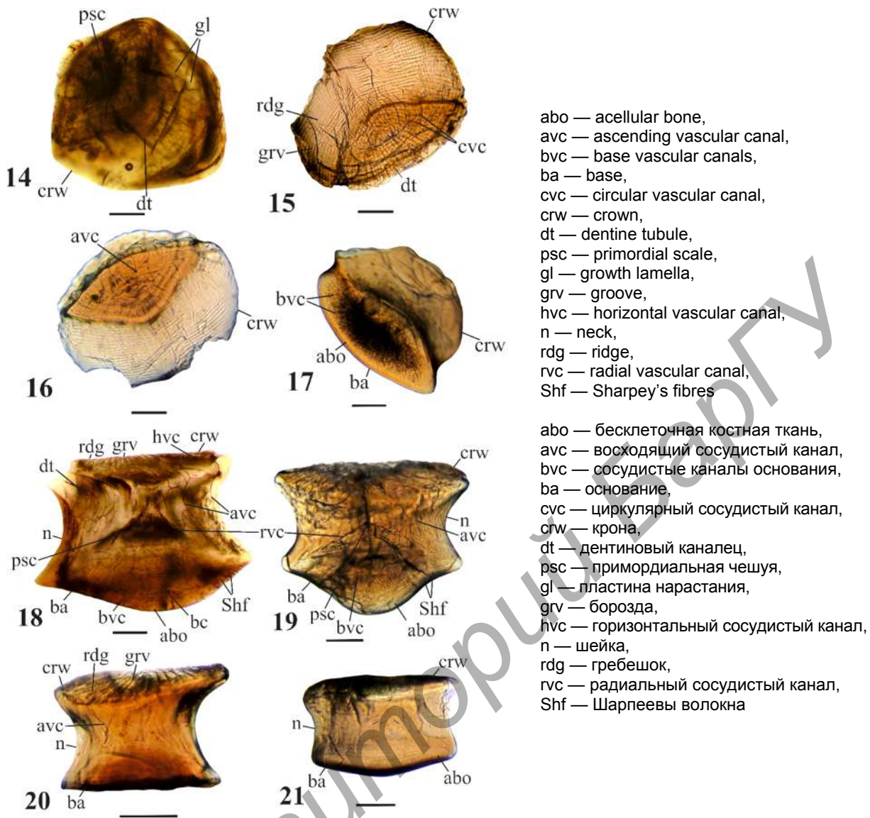
Figures 14–21 — Microstructure of the scales of Diplacanthus kleesmentae : 14 — horizontal section of the scale crown. Specimen No 121/44–19, Korma 1 borehole, depth 340.2 m, Vitebsk Regional Stage, Lepel Beds; 15 — horizontal section of the scale crown. Specimen No 121/44–25, Korma 1 borehole, depth 340.2 m, Vitebsk Regional Stage, Lepel Beds; 16 — scale horizontal view in anise oil. Specimen No 143/30–46, Klimovichi 4n borehole, depth 487.8 m, Vitebsk Regional Stage, Obol Beds. 17 — horizontal view of the base in anise oil. Specimen No 143/30–48, Klimovichi 4n borehole, depth 487.8 m, Vitebsk Regional Stage, Obol Beds; 18 — scale vertical longitudinal section. Specimen No 121/44–20, Korma 1 borehole, depth 340.2 m, Vitebsk Regional Stage, Lepel Beds; 19 — scale vertical longitudinal view in anise oil. Specimen No 143/30–47, Klimovichi 4n borehole, depth 487.8 m, Vitebsk Regional Stage, Obol Beds; 20 — scale lateral view in anise oil. Specimen No 121/44–27, Korma 1 borehole, depth 340.2 m, Vitebsk Regional Stage, Lepel Beds; 21 — scale lateral view in anise oil. Specimen No 143/30–46, Klimovichi 4n borehole, depth 487.8 m, Vitebsk Regional Stage, Obol Beds. Scale bar of 200 \mu\text{m} ( 14–21 )
