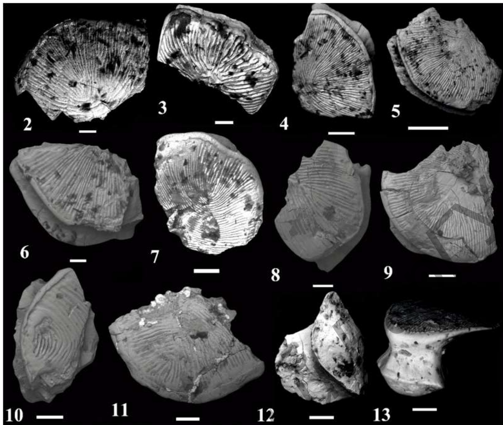
Figures 2—13 — Acanthodian scales of Diplacanthus kleesmentae from the Upper Emsian of the Lower Devonian of Belarus: 2 — Specimen No 116/51–1, Bykhov 1 borehole, depth of 321.5 m, \times 100 scale, crown view; Vitebsk Regional Stage, Lepel Beds; 3 — Specimen No 116/53–1, Bykhov 1 borehole, depth of 324.2 m, \times 140 , scale, crown view; Vitebsk Regional Stage, Lepel Beds; 4 — Specimen No 121/44–6, Korma 1 borehole, depth of 340.2 m, \times 85 , scale, oblique crown view; Vitebsk Regional Stage, Lepel Beds; 5 — Specimen No 121/44–3, Korma 1 borehole, depth of 340.2 m, \times 50 , scale, oblique crown view; Vitebsk Regional Stage, Lepel Beds; 6 — Specimen № 143/30–17, Klimovichi 4п borehole, depth of 487.8 m, \times 100 , scale, oblique crown view; Vitebsk Regional Stage, Obol Beds; 7 — Specimen No 143/30–18, Klimovichi 4п borehole, depth of 487.8 m, \times 200 , scale, oblique crown view; Vitebsk Regional Stage, Obol Beds; 8 — Specimen No 143/30–37, Klimovichi 4п borehole, depth of 487.8 m, \times 120 , scale fragment, oblique crown view; Vitebsk Regional Stage, Obol Beds; 9 — Specimen No 143/30–41, Klimovichi 4п borehole, depth of 487.8 m, \times 90 , scale, crown view; Vitebsk Regional Stage, Obol Beds; 10 — Specimen № 143/30–44, Klimovichi 4п borehole, depth of 487.8 m, \times 150 , scale fragment, oblique crown view; Vitebsk Regional Stage, Obol Beds; 11 — Specimen № 143/31–1, Klimovichi 4п borehole, depth of 489.8 m, \times 130 , scale fragment, crown view; Vitebsk Regional Stage, Obol Beds; 12 — Specimen № 121/44–1, Korma 1 borehole, depth of 340.2 m, \times 75 , scale, basal view; Vitebsk Regional Stage, Lepel Beds. 13 — Specimen № 121/44–5, Korma 1 borehole, depth of 340.2 m, \times 70 , scale, lateral view; Vitebsk Regional Stage, Lepel Beds. Scale bar 100 \mu\text{m} (2, 3, 6, 8, 10, 11); 200 \mu\text{m} (4, 7, 9, 12, 13); 500 \mu\text{m} (5)
